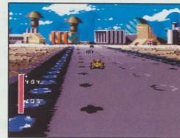
Scroll Locked
