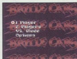
Mode Screen
