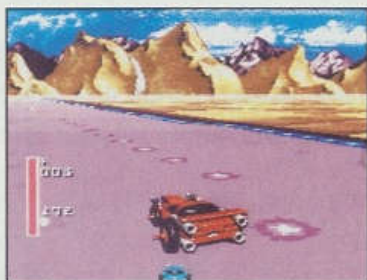
Boss Radar
