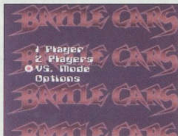
Vs. Mode
