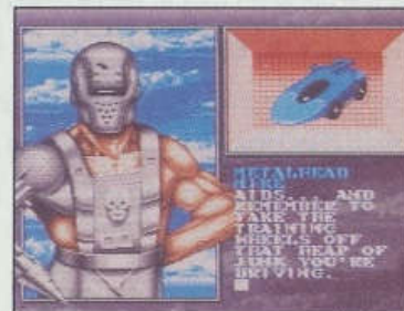
Boss Screen
